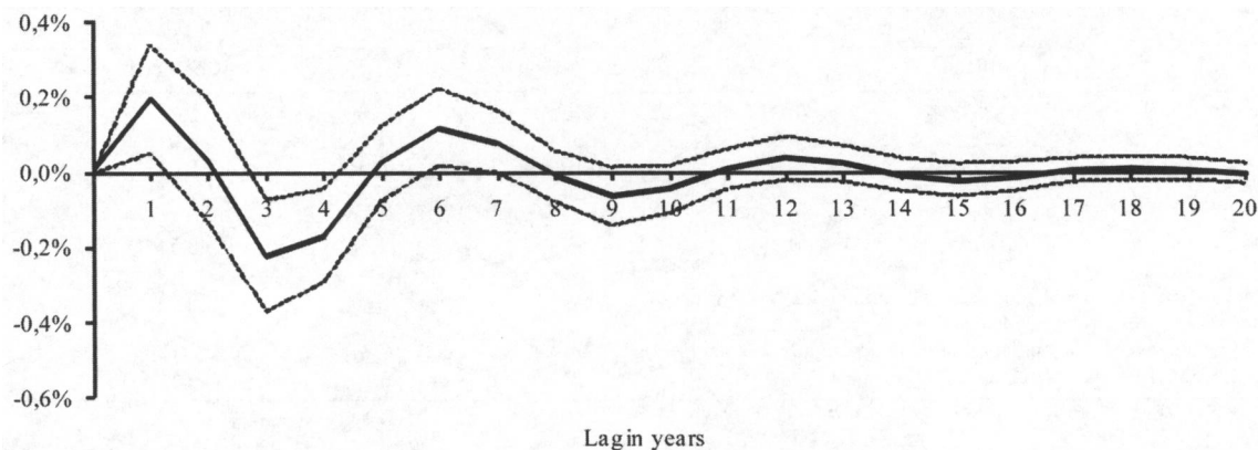
FIGURE 2.—EFFECT OF A SHOCK IN BUSINESS OWNERSHIP (1%) TO REAL GDP, HP-FILTERED DATA ( \lambda = 6.25 )
